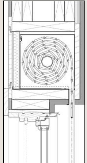
In Wall - When planned during the pre-construction phase, shutters can be installed in wall, hiding the box and rails for a near invisible application when the shutters are rolled up.
