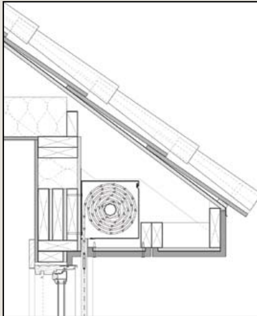
In Soffit - Allows the box to be hidden for a lower profile shutter.
