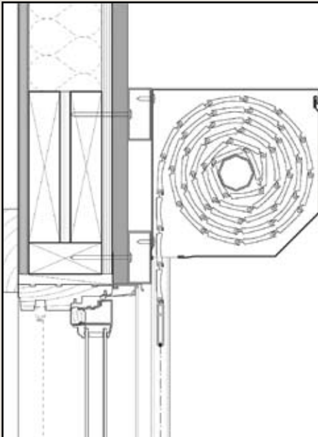
Retrofit - Installation outside the building.
