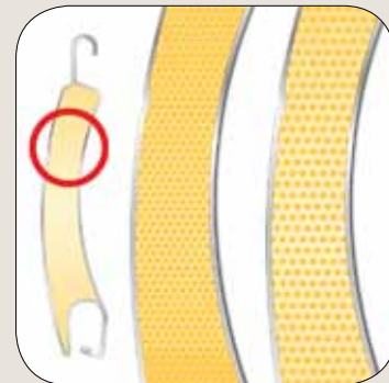
Detail of the RLL59 Slat
